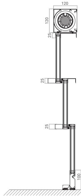
3 - Sash Vertical Sliding system
