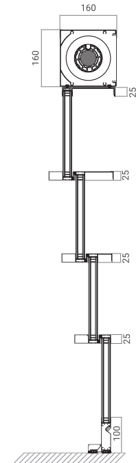
4 - Sash Vertical Sliding system
